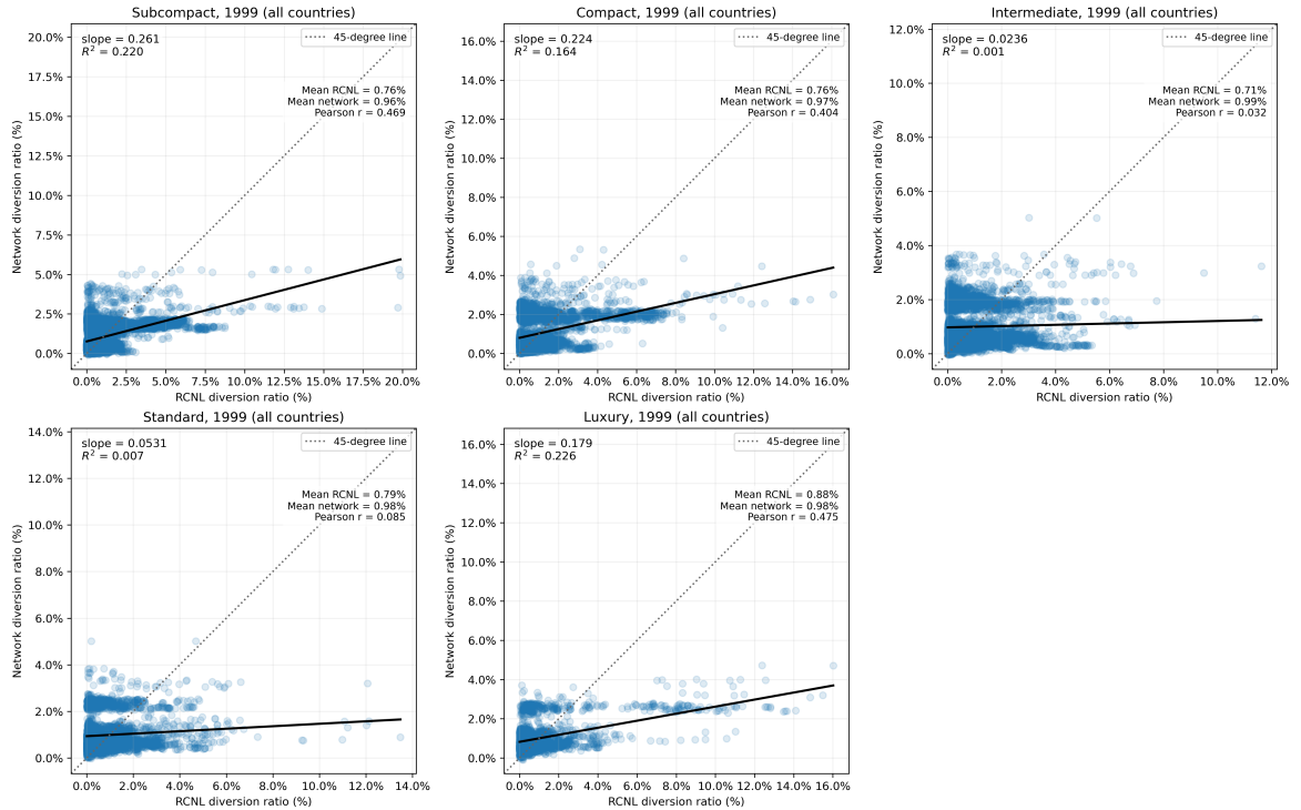
Figure D.1: Comparison between diversion ratios in the RCNL and the Network model.
