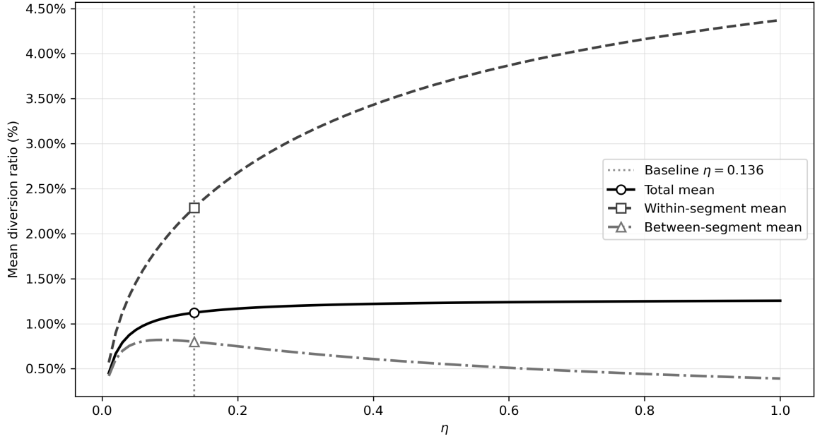
Figure D.2: Average Diversion Ratio for Different Values of \eta
